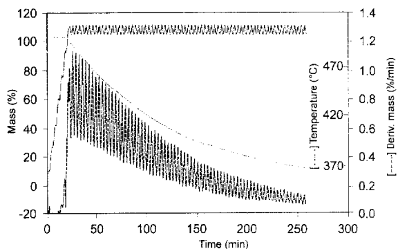
Fig. 3 Quasi-isothermal profile for polytetrafluoroethylene
