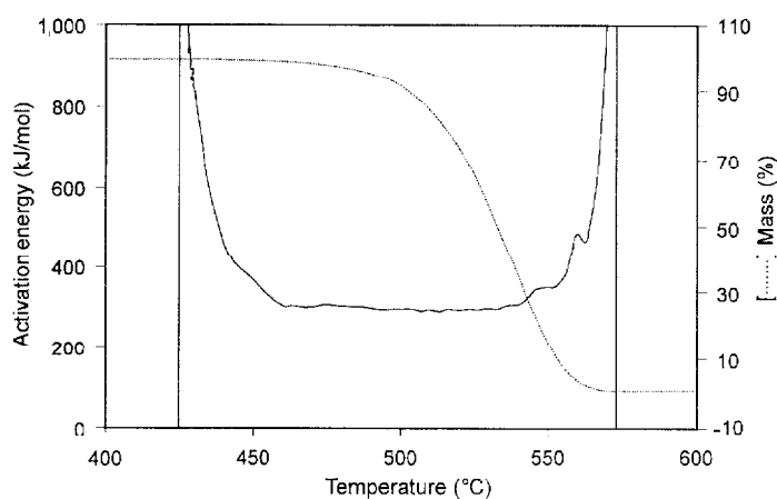
Fig. 2 Activation energy for polytetrafluoroethylene
