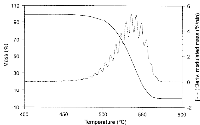
Fig. 1 Modulated temperature profile for polytetrafluoroethylene
