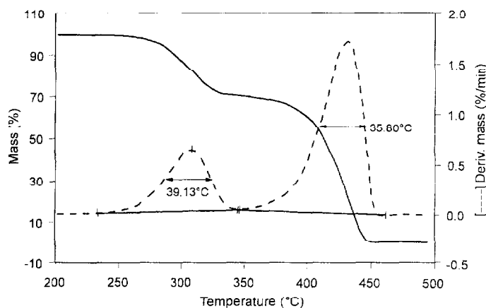
Fig. 6 Determination of full width temperature at half height.
