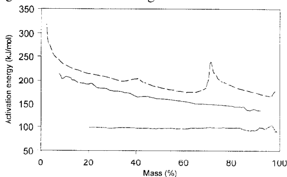
Fig. 5 Effect of conversion on activation energy. — — poly (60% ethylene vinyl acetate); — polystyrene; - - - 1,4-diphenylbutadiene
