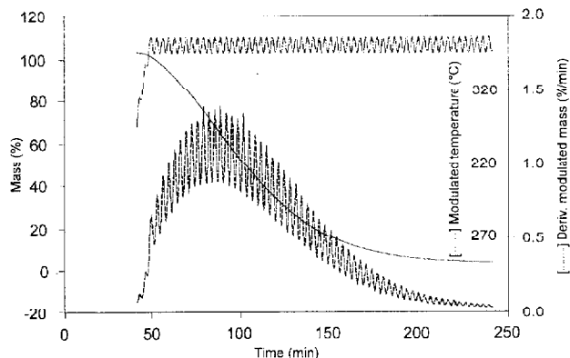
Fig. 4 Quasi-isothermal profile for polystyrene
